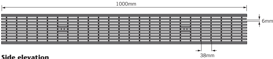
Side elevation
