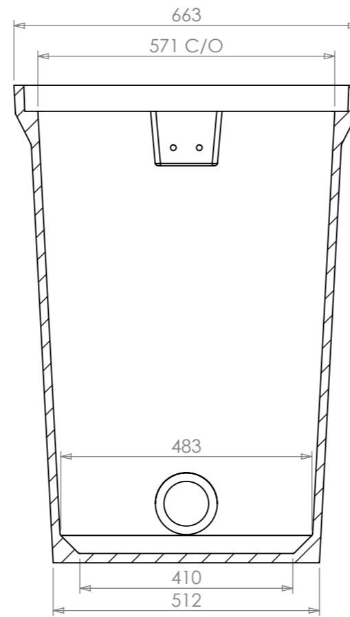
SECTION B-B
